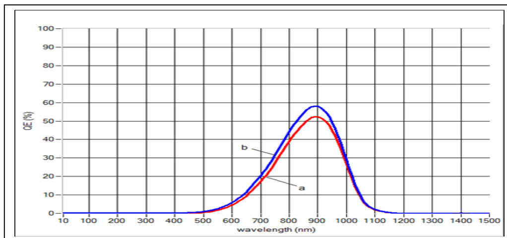
Figure (3): The effect of n-region concentration a- 1 \times 10^{14} , b- 1 \times 10^{16}/\text{cm}^3 . With n_p dopant 10^{14} and indium concentration 10^{14} , T_{h_n} = 100\mu\text{m} , T_{h_p} = 20\mu\text{m} .
